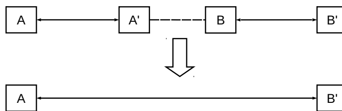
Fig. 5. Schematic structure of a quantum repeater.
