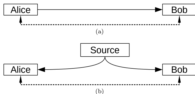
Fig. 1. (a) Prepare-and-measure protocol (e.g. BB84 [30]), (b) Entanglement-based protocol (e.g. E91 [35]). Solid line denotes the quantum channel, dashed line stands for the authenticated classical channel. Arrows denote the direction of information flow.
